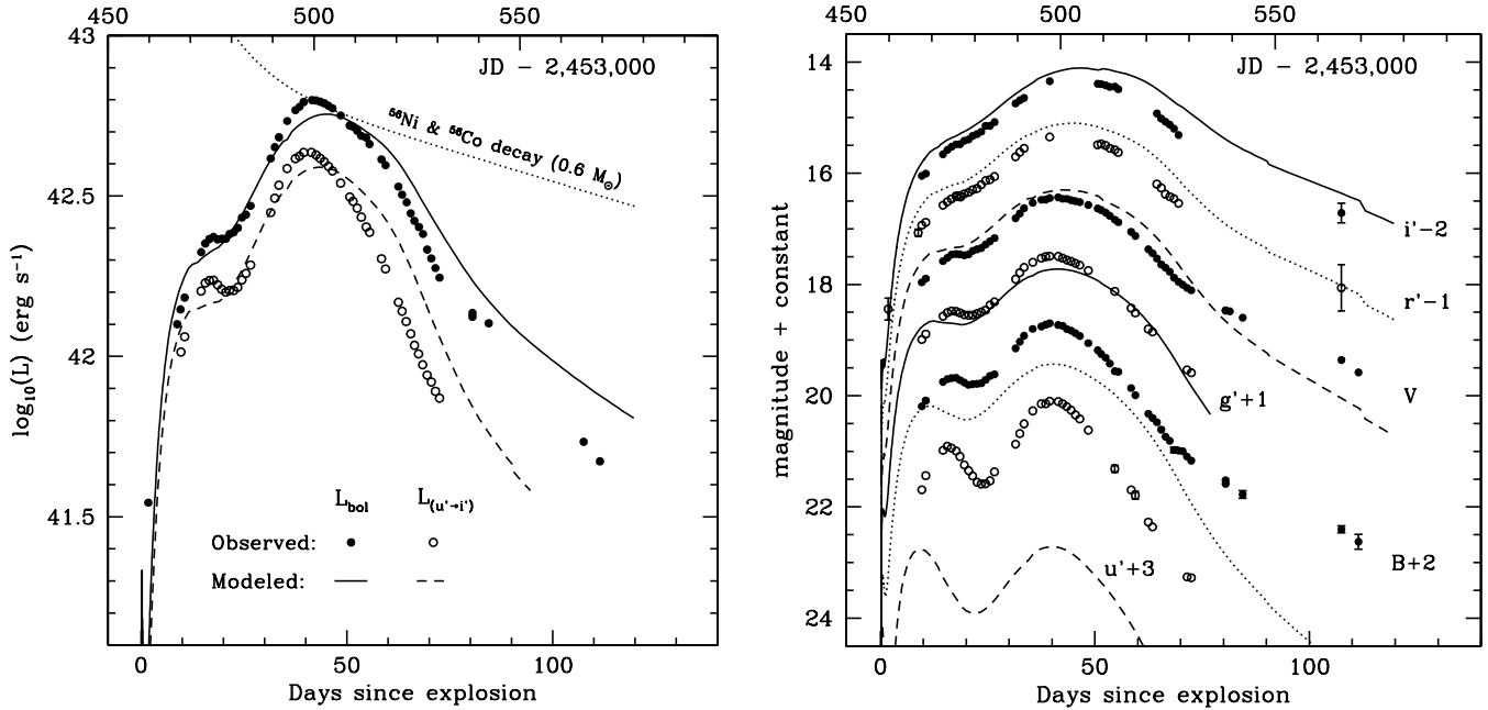
FIG. 10.— Left : Modeled bolometric ( solid line ) and UVOIR ( dashed line ) luminosities of the mixed 8.29 M_{\odot} WN star explosion. The circles mark the UVOIR luminosity L_{u'-i'} ( open ) and the bolometric luminosity L_{\text{bol}} ( closed ), as derived from the observations. The dotted line shows the predicted luminosity if the ejecta were able to trap the entire \gamma -ray output of 0.6 M_{\odot} of radioactive ^{56}\text{Ni} produced in the explosion. The time of outburst was assumed to be JD 2,453,458. Right : Modeled u'g'r'i'BV light curves ( lines ) compared with the observations ( circles ).
