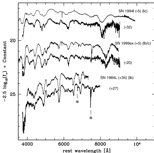
FIG. 5.—Comparison of spectra of SN 2005bf with those of other Type Ib and Ic SNe. At the top, the spectrum from day -32 compared with that of the Type Ic SN 1994I 5 days before maximum light (Filippenko et al. 1995). At the middle, the spectrum from day -20 and that of the Type Ib/Ic SN 1999ex 5 days after maximum light (Hamuy et al. 2002). At the bottom, the spectrum from day +27 and that of the Type Ib SN 1984L 34 days after maximum light (Harkness et al. 1987). Telluric features are marked with an Earth symbol.
