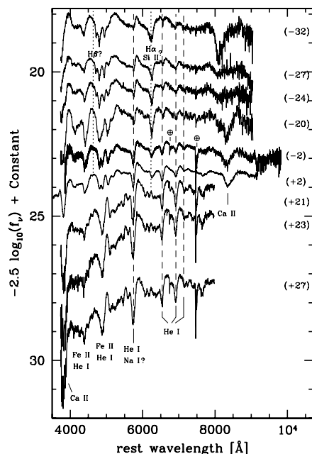
FIG. 4.—Spectroscopic evolution of SN 2005bf. Each spectrum is presented on a logarithmic scale, shifted by an arbitrary constant. The wavelength of the spectra was shifted to the SN rest frame using a redshift of z = 0.01833 . The labels in parentheses to the right of each spectrum indicate the epoch in rest-frame days since L_{\text{bol}} maximum (JD = 2,453,499.8). The spectrum from day -20 was smoothed by averaging over 5 pixels. The name of the ions responsible for some of the main features are given. The dotted vertical lines mark the wavelength at which the minimum of the H \alpha and H \beta lines would appear if hydrogen were present at \sim 14,500 km s -1 . The dashed vertical lines mark the absorptions due to He I \lambda\lambda 5876, 6678, 7065, 7281 , at an expansion velocity of \sim 6000 km s -1 . Telluric features are marked with an Earth symbol (⊕).
